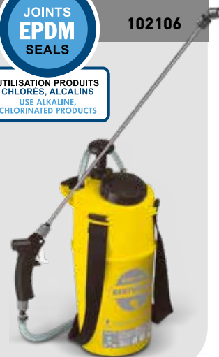
Fixed and off-centre pressurizing pump. Stainless steel rod
